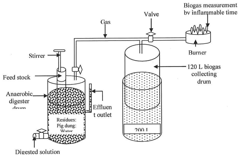
Figure1. Diagram of a floating drum digester
